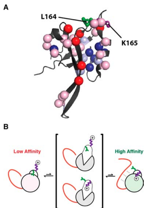
Figure 7. Segregation of dynamic and stable subdomains suggests a possible mode of partial PDZ unfolding. (A) Pink spheres indicate residues with R_{\text{ex}} \geq 2 \text{ s}^{-1} in CRIB-PDZ 130–255 and PDZ 156–255 and red spheres indicate R_{\text{ex}} \geq 2 \text{ s}^{-1} and those residues globally fit for both. Light-blue and navy spheres indicate residues with detectable protection factors (the ‘folding core’), where the latter concurrently lack R_2 dispersions. One residue, V239, is colored violet because it has a detectable protection factor and significant R_{\text{ex}} . (B) Schematic of L/K switch isomerization via a partial unfolding mechanism. Residue L164 is colored green, and K165 is colored purple. Brackets surrounding two center diagrams represent putative energetically equivalent states in the folding intermediate state. CRIB domain is colored red.
