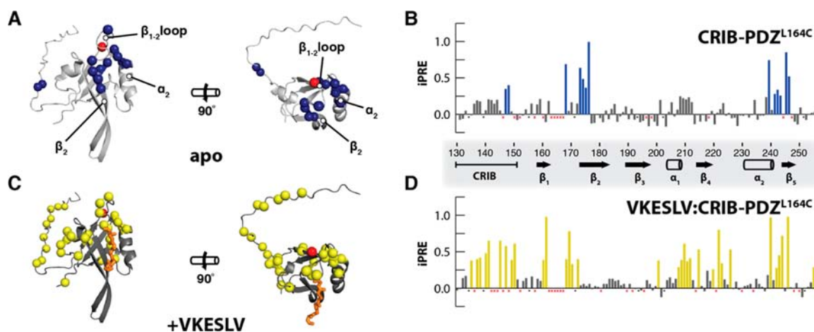
Figure 2. VKESLV binding flips the L/K switch. PRE data for CRIB-PDZ L164C . (A) Blue spheres indicate broadened residues in the apo state. (B) iPRE (iPRE = 1 - I^{para}/I^{dia} ) vs residue number for CRIB-PDZ L164C . Residues with significant iPRE values include: A147 and I148 of the CRIB domain, S168 of the \beta_{1-2} loop; G174, F174, Y165, and I176 of the \beta_2 strand; and V239, N241, S242, and S243 of the \alpha_2 helix, and L245 and I246 of the \beta_6 strand. (C) Yellow spheres indicate broadened residues in VKESLV-bound state (VKESLV:CRIB-PDZ L164C ratio \geq 6:1 ), where blue bars indicate those with proximity to MTSL attached to C164 side chain. (D) iPRE vs residue number for CRIB-PDZ L164C and VKESLV:CRIB-PDZ L164C , where yellow bars indicate those with proximity to MTSL attached to C164 side chain. Significant iPREs for the CRIB domain (S135, S137, I138, H140, D141, V145, A147, I149, D150), \beta_1 strand (R160, V161), \beta_{1-2} loop (S168, D169, K170, L172), \beta_{2-3} hairpin (L200), \alpha_1 helix region (E207, S208, T209, G210, L211, V214), \beta_{4-5} region (I219, V221, N222, K229), \alpha_2 helix (N241, S242, S243), and \beta_6 strand (I246) highlight a surface of the PDZ domain distant from the binding cleft (C,D). C164 is marked by a red sphere in (A,C). Proline residues are marked with a black asterisk, and residues without a calculated iPRE value are marked with a red “x”. A complete list of iPRE by residue for apo and VKESLV-bound states is located in Table S1.
