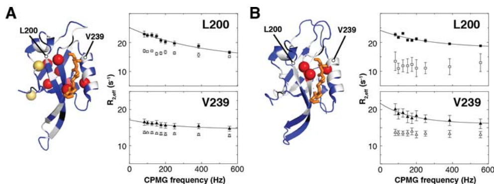
Figure 6. VKESLV binding quenches R_{\text{ex}} in PDZ ^{156-255} and CRIB-PDZ ^{\text{Q144C/L164C}} . Comparison of CPMG-based R_2 relaxation dispersion data for apo and VKESLV-bound PDZ ^{156-255} and CRIB-PDZ ^{\text{Q144C/L164C}} . White spheres represent quenched dispersions for VKESLV-bound Par-6 relative to apo state, red spheres those that retain dispersions, and yellow for dispersions detected only in VKESLV:PDZ ^{156-255} are indicated in for (A) VKESLV:PDZ ^{156-255} and (B) VKESLV:CRIB-PDZ ^{\text{Q144C/L164C}} . Nonexchanging residues are colored blue. Representative dispersion curves demonstrating reduced R_{\text{ex}} upon VKESLV binding for both where black and white circles represent data for L200 in the apo and VKESLV-bound state, respectively. Black and white triangles represent data for V239 in the apo and VKESLV-bound state, respectively. VKESLV:protein ratio is 6:1. Analysis proceeded as described previously. ^1
