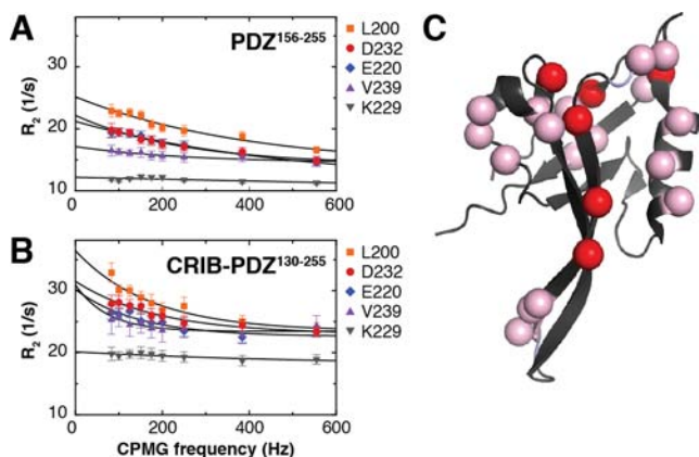
Figure 3. ^{15}\text{N} relaxation dispersion reveals a domain-wide transition in apo PDZ ^{156-255} and CRIB-PDZ ^{130-255} . Representative dispersion curves for several sites of (A) PDZ ^{156-255} and (B) CRIB-PDZ ^{130-255} as well as sites that lack dispersion and possess a flat, featureless profile as a result. 1/\tau_{\text{cp}} is the effective B_1 frequency in the CPMG experiment. (C) Pink spheres indicate residues with significant \mu\text{s} – \text{ms} exchange for both PDZ ^{156-255} and CRIB-PDZ ^{130-255} . Red spheres indicate residues with significant individual \mu\text{s} – \text{ms} exchange and those globally fitted for both PDZ ^{156-255} and CRIB-PDZ ^{130-255} . Analysis proceeded as described previously. 1
