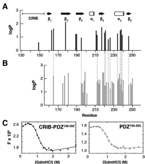
Figure 5. Par-6 CRIB destabilizes the PDZ. Native ^1\text{H} - ^2\text{D} exchange data by residue for (A) CRIB-PDZ ^{130-255} (black bars) and (B) PDZ ^{156-255} (gray bars) at 25 °C. Dashed lines connect residues that exhibit significant protection factors ( \log P ) for both proteins. (C) Equilibrium guanidine denaturation measurements with increasing concentrations of GdnHCl. Curves represent fitted functions used to determine \Delta G_{\text{GdnHCl}} . Open circles represent PDZ ^{156-255} ( \Delta G_{\text{unf}}^{\text{PDZ}} = 3.2 \pm 0.3 kcal/mol), and black diamonds signify CRIB-PDZ ^{130-255} ( \Delta G_{\text{unf}}^{\text{CRIB-PDZ}} = 2.8 \pm 0.4 kcal/mol).
