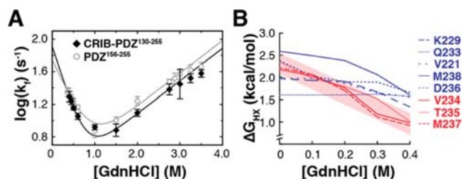
Figure 4. An intermediate is detectable in Par-6 unfolding. (A) Single-jump stopped-flow chevron plots for CRIB-PDZ ^{130-255} (black diamonds) and PDZ ^{156-255} (gray circles). Both chevrons display slight rollover in the unfolding arm. Nonlinearly fitted two-state folding equations are shown with black and gray lines for CRIB-PDZ ^{130-255} and PDZ ^{156-255} , respectively. (B) ^1\text{H} – ^2\text{D} exchange vs [\text{GnHCl}] graph showing CRIB-PDZ ^{130-255} residues. V234, T235, and M237 respond linearly to low [\text{GnHCl}] , indicating their proximity to the region disrupted upon formation of the folding intermediate, and are colored red. All other residues are colored blue.
